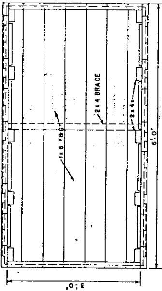
PLAN
