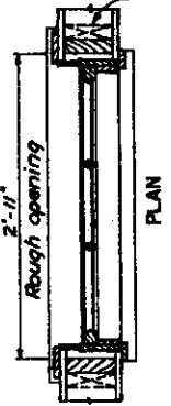
TILTING SASH (STOCK FRAME)
