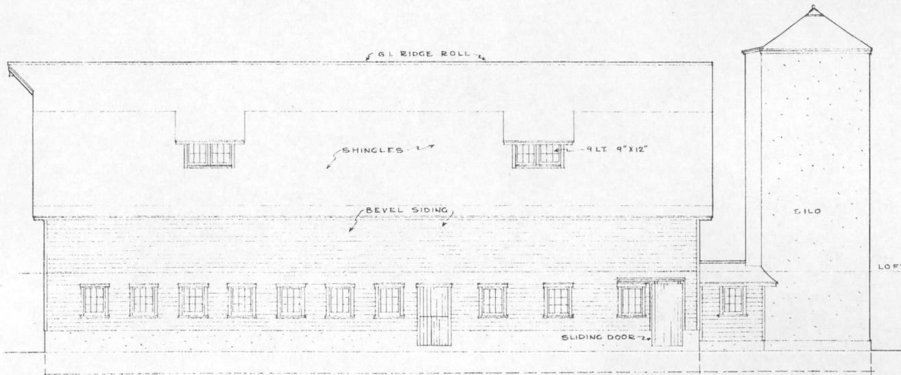
EAST ELEVATION SCALE \frac{1}{8}'' = 1'-0''
