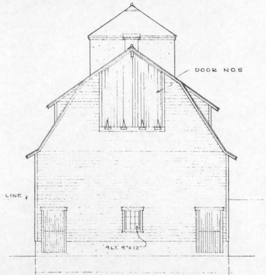
SOUTH ELEVATION SCALE \frac{1}{8}'' = 1'-0''
