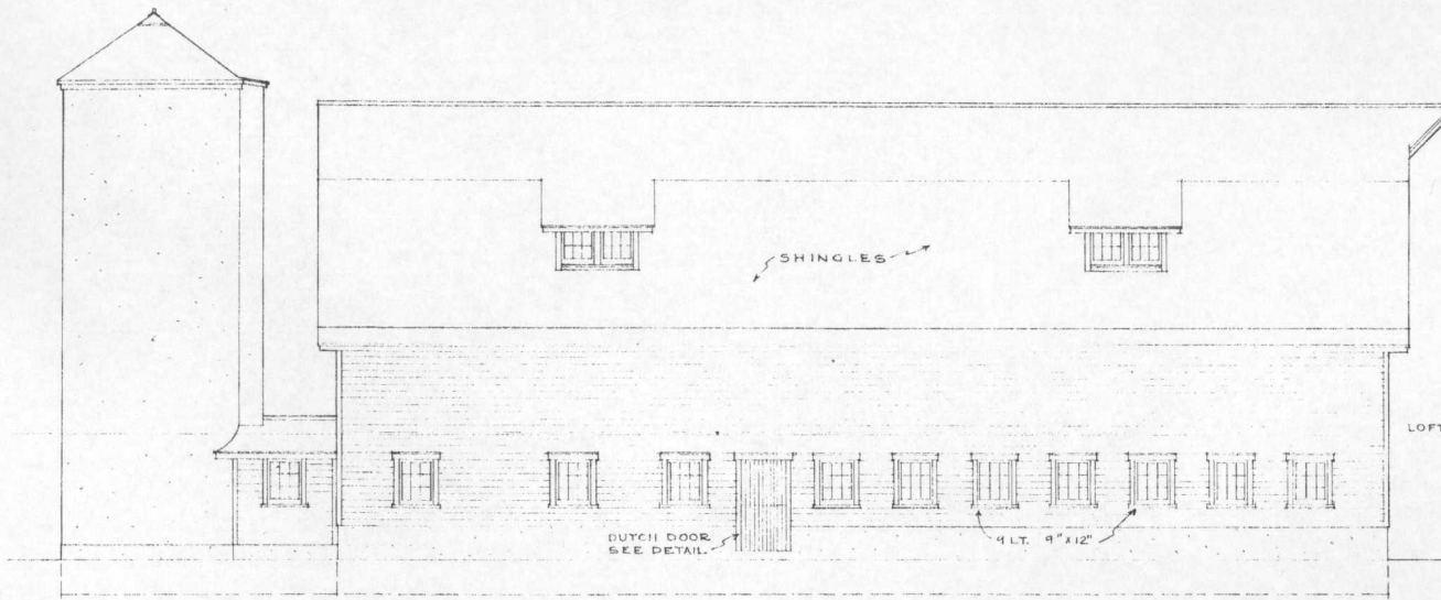
WEST ELEVATION SCALE \frac{1}{8}'' = 1'-0''
