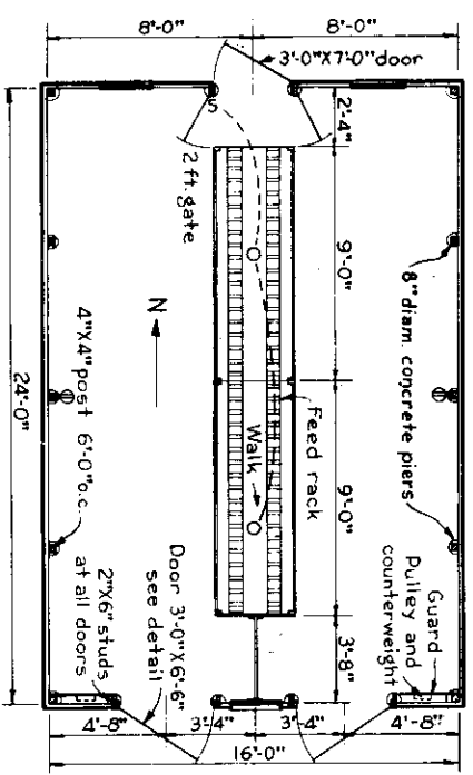
PLAN Scale 1/2" = 1'-0"
