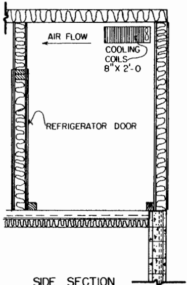
SIDE SECTION
