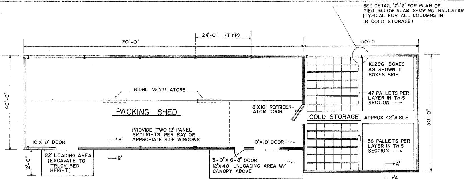
FLOOR PLAN
