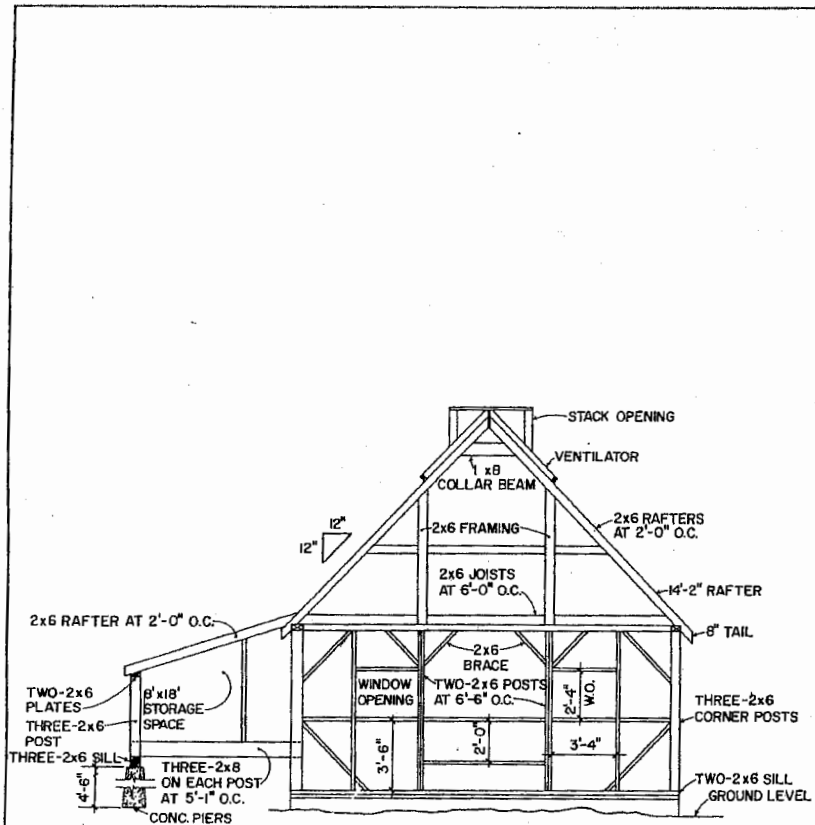
NORTH END FRAMING SCALE: 0 1 2 3 4 12' 6" 9"
