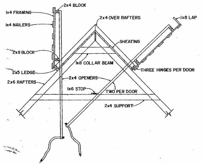
SECTION THROUGH VENTILATOR SCALE: 0 1 2 3 12' 6" 9"
