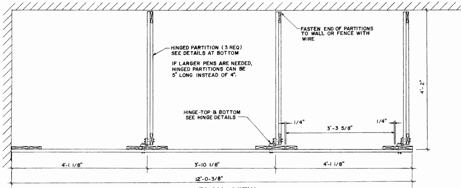
PLAN VIEW
