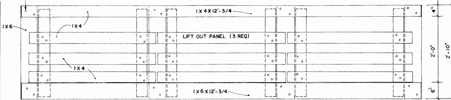
ELEVATION VIEW
