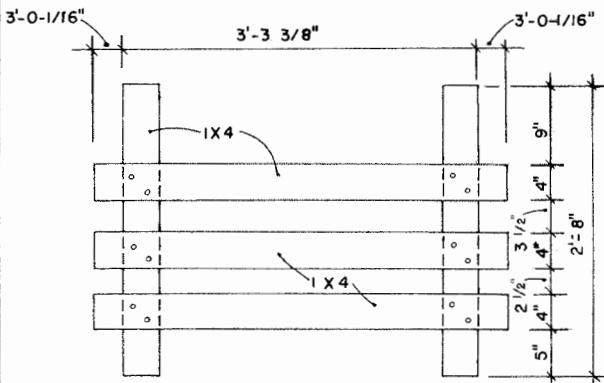
LIFT OUT PANEL DETAILS
