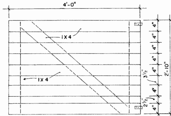
PARTITION DETAILS
