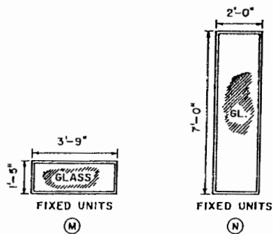
WINDOW SCHEDULE
