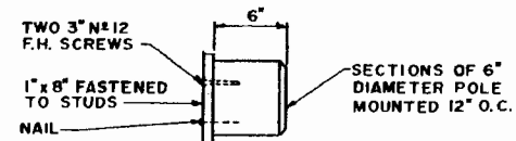
BRIDLE RACK
