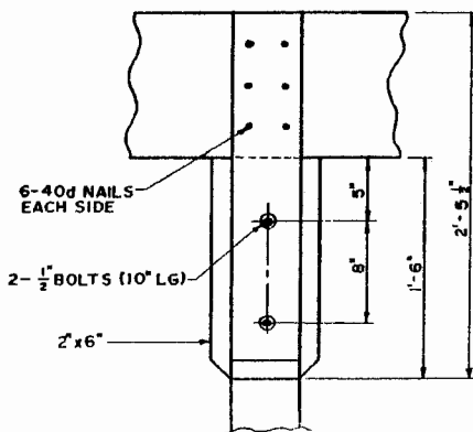
POST & GIRDER DETAIL
