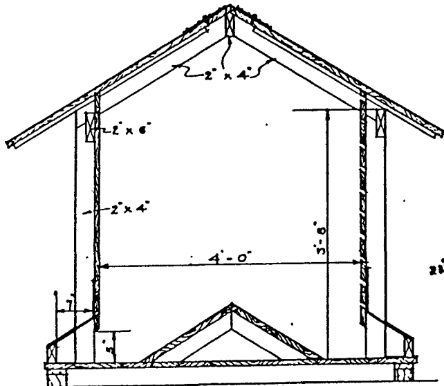
·CROSS SECTION· ·EAR CORN SELF FEEDER·
