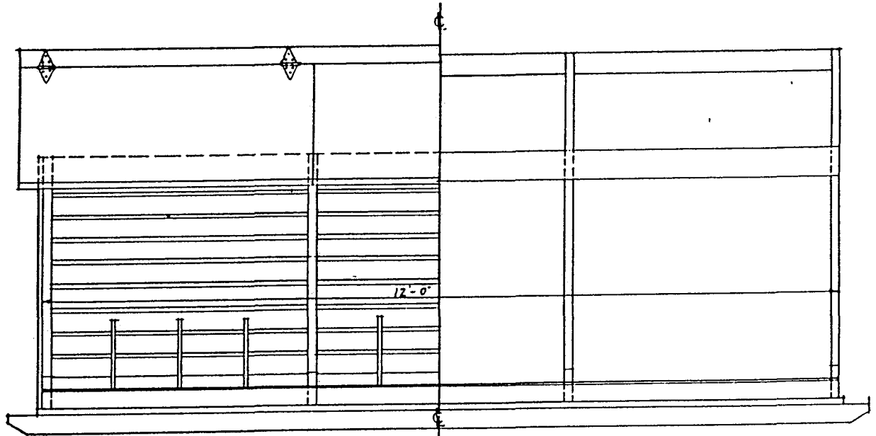
ASSEMBLY · FRONT ELEVATION · FRAMING · EAR CORN SELF FEEDER ·
