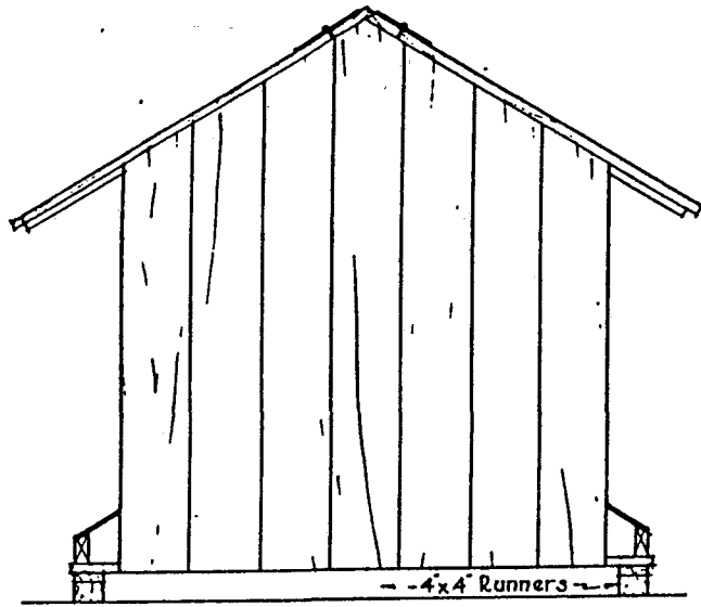
·END ELEVATION· ·EAR CORN SELF FEEDER·
