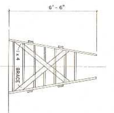
BRACING DETAIL
