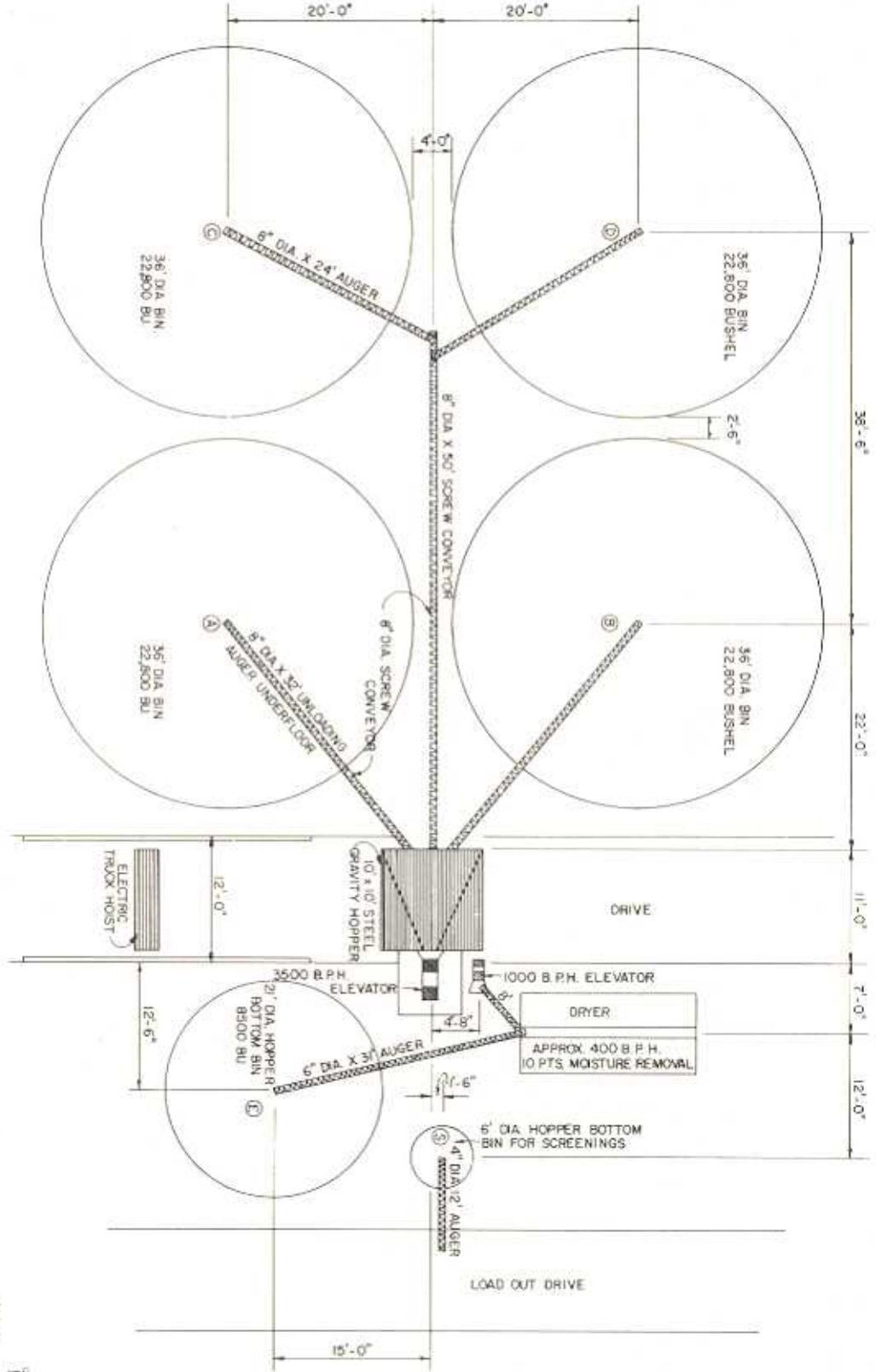
PLAN VIEW
